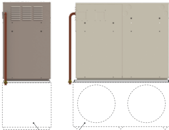
Existing supply/return air plenum box.
